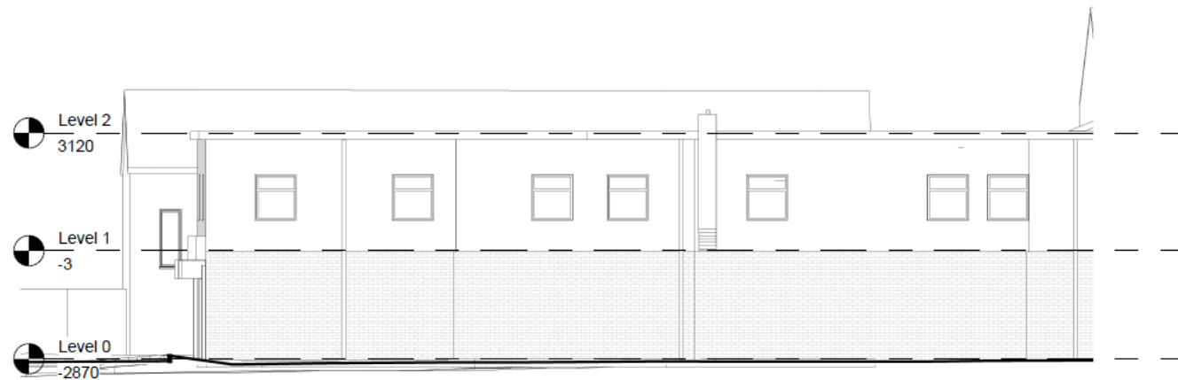
REAR ELEVATION
